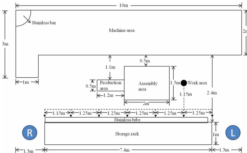
Figure 8. As-Is factory layout. (The notation R and L are mapping to the Figure 7 storage rack direction).
